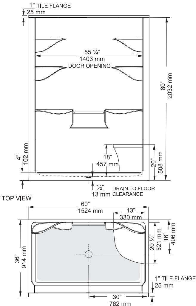
CENTRE DRAIN - LEFT HAND SHOWER SHOWN FRONT VIEW
